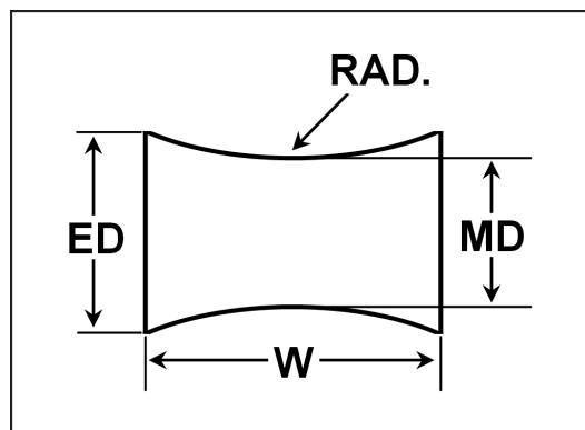
Wide concave roller diagram
