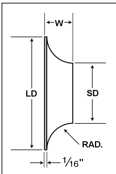
Concave bevel stitcher diagram
