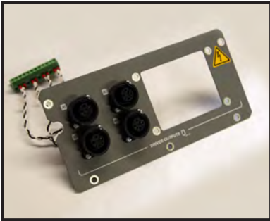
◀ RELAY PANEL ASSEMBLY ELECTRIC HEATER MODULE ▶
