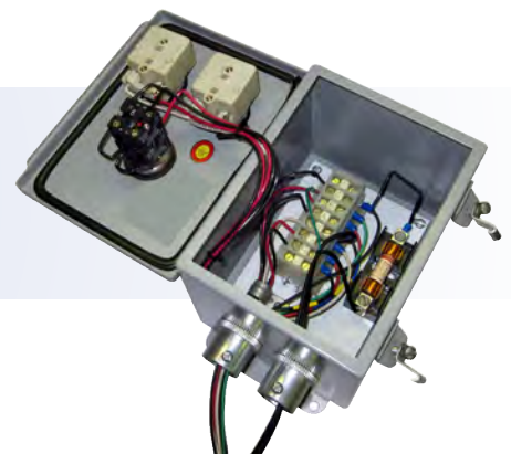
◀ ELECTRO-MECHANICAL ASSEMBLY ELECTRIC CONTROL BOX ▶
